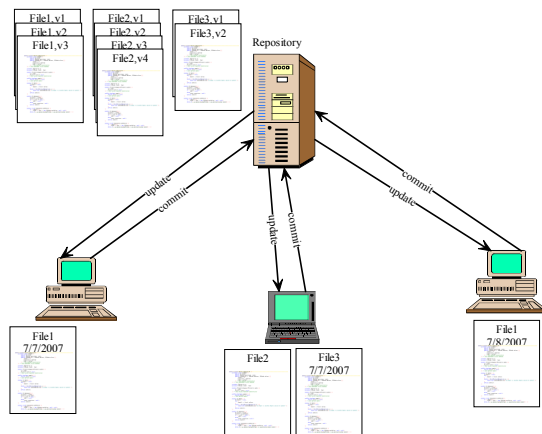
Figure 1 - Source Manager Server
