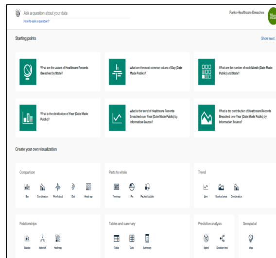
Figure 1. Watson Analytics Discovery Screen
